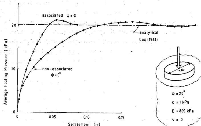
Fig. 2.2 Finite element results for plate indentation; the limit load does not depend on the dilatancy angle \psi .
