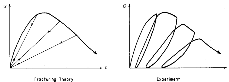
Fig. 9.1 Dougill's theory exaggerates the degradation of the unloading-reloading modulus.
