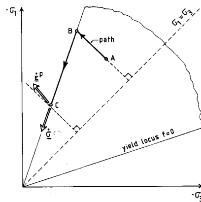
Fig. 5.2 The negativeness of \dot{\sigma}^T \dot{\varepsilon}^p and \dot{\sigma}^T \dot{\varepsilon} explains the unstable lower curve in Fig. 5.1.
