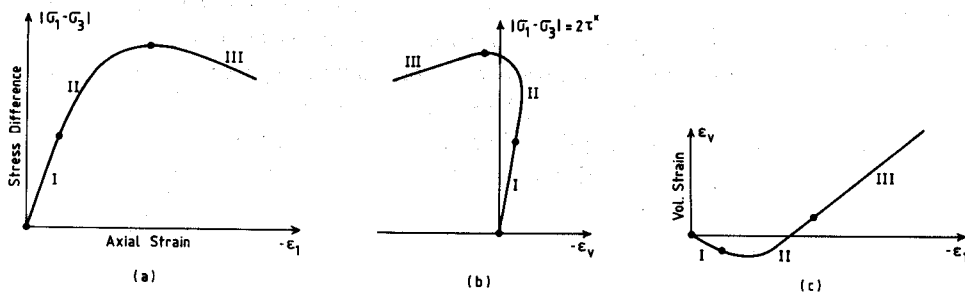
Fig. 3.2 Typical triaxial test results for a loose or a cemented granular material.
