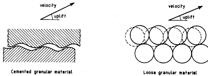
Fig. 3.4 Sliding at microcracks and sliding between groups of particles; both cases give dilation.
