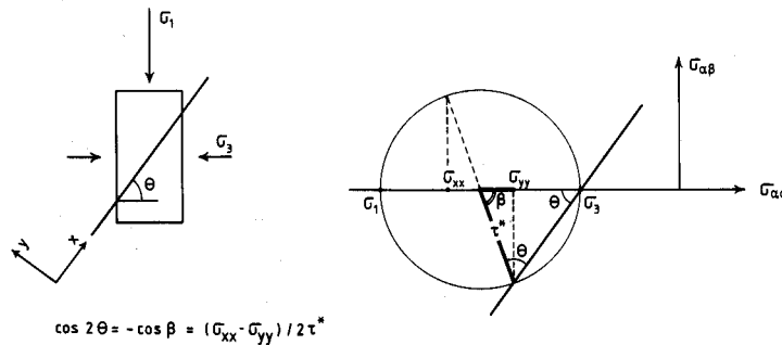
Fig. 8.6 Inclination angle and Mohr's stress circle.
