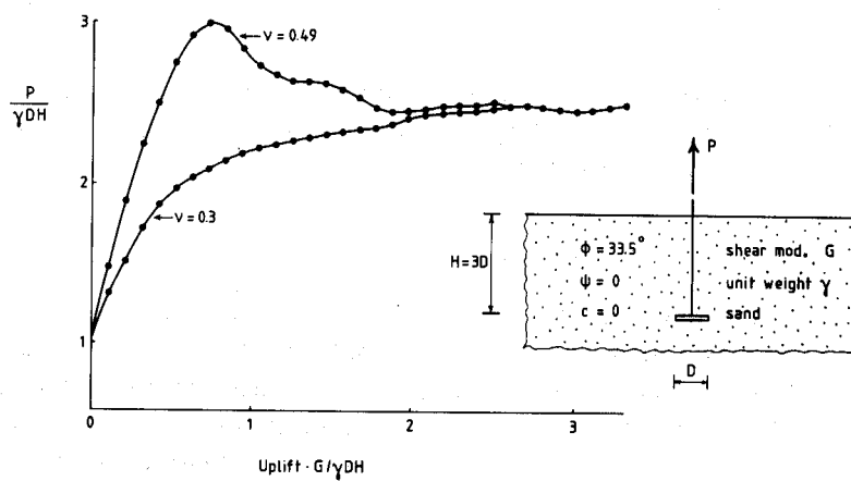
Fig. 5.5 Finite element results for an anchor in sand; the limit load depends on Poisson's ratio.
