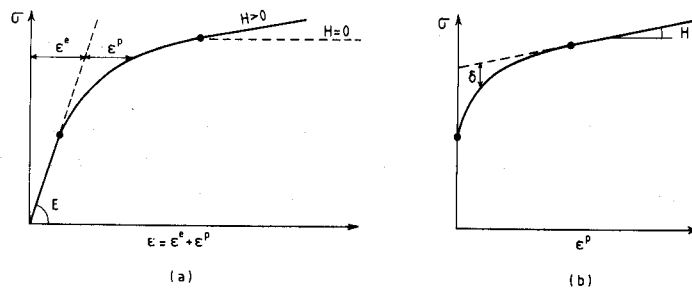
Fig. 9.2 The hardening modulus is calculated from the distance \delta and the ultimate value H , which can be zero.
