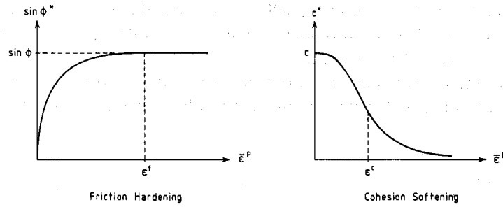
Fig. 7.2 Quasi-empirical relations in the hardening-softening model.
