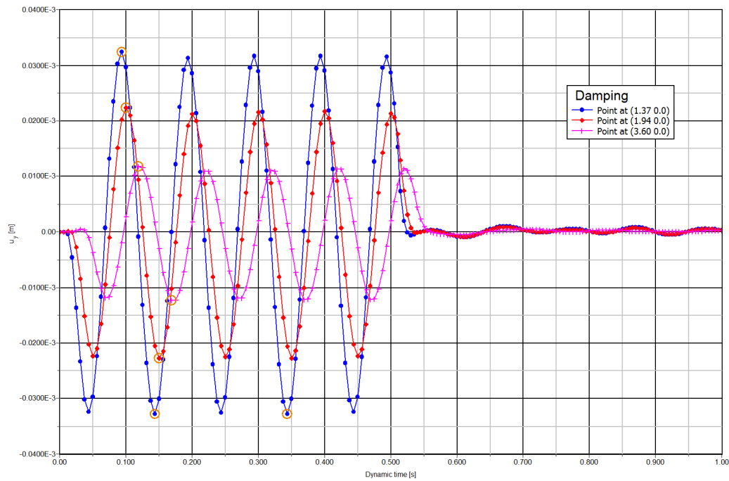
Figure 199: Vertical displacement vs time on the surface at different distances to the vibrating source (with damping)
