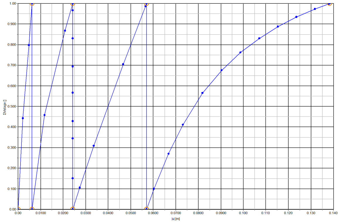
Figure 56: Load-displacement curve of deflection of wall
