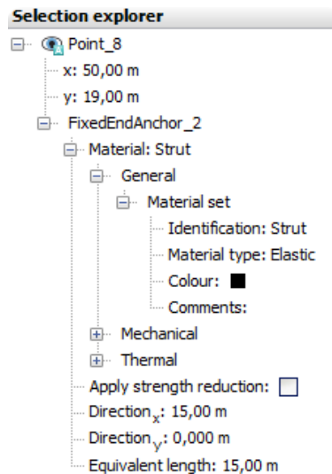
Figure 45: Parameters for fixed-end anchors in the Selection explorer
