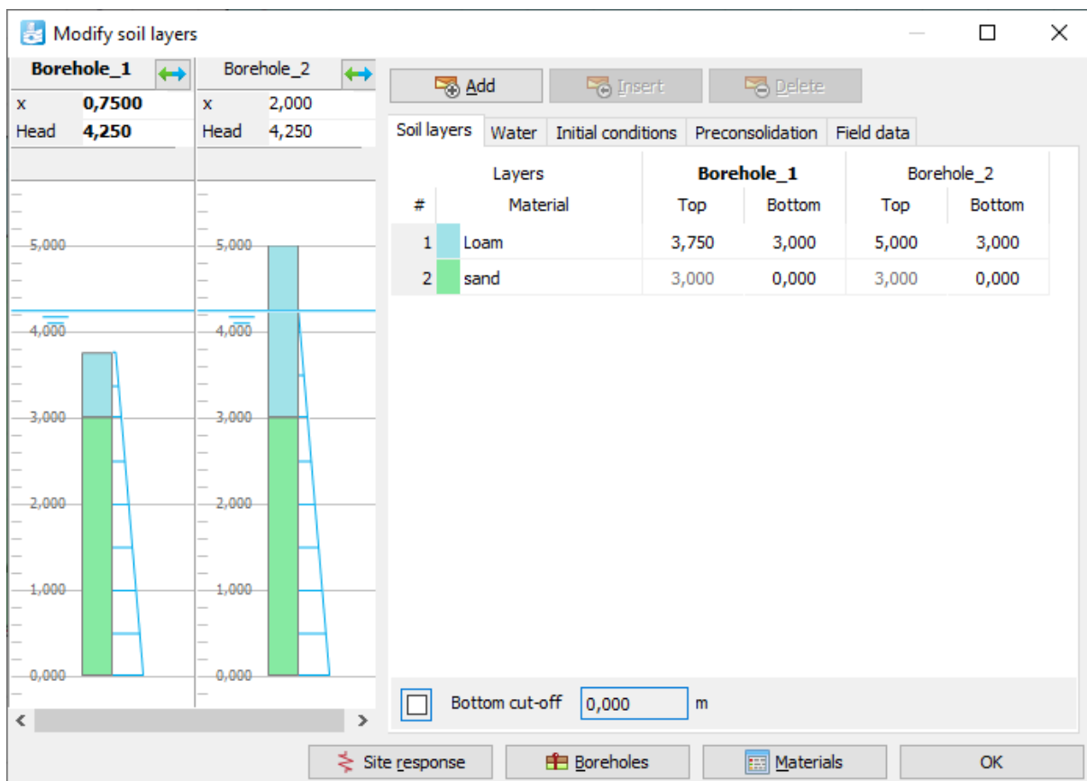
Figure 164: Soil stratigraphy in the Modify soil layers window
