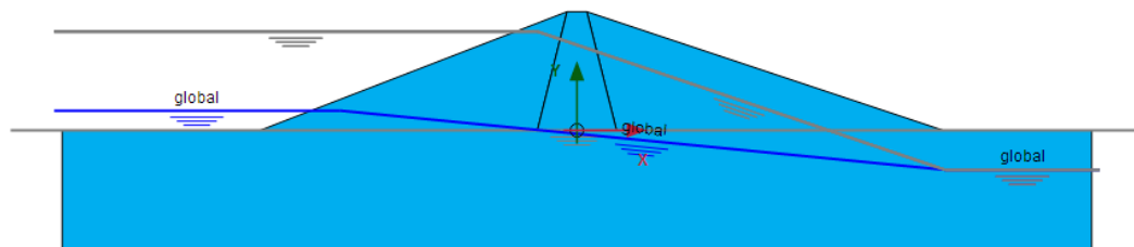
Figure 183: Model for the low level case in the Flow conditions mode
