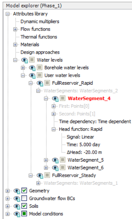
Figure 180: Properties of the lowering water segment
