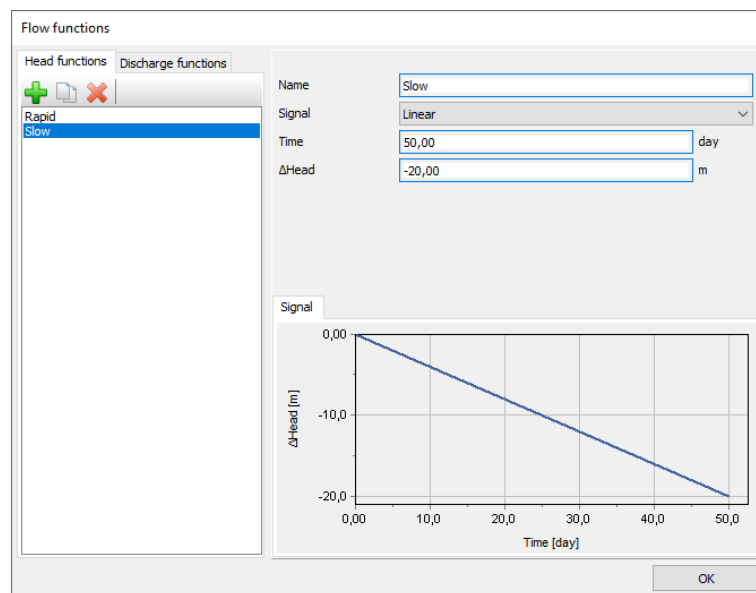
Figure 182: The flow function for the slow drawdown case
