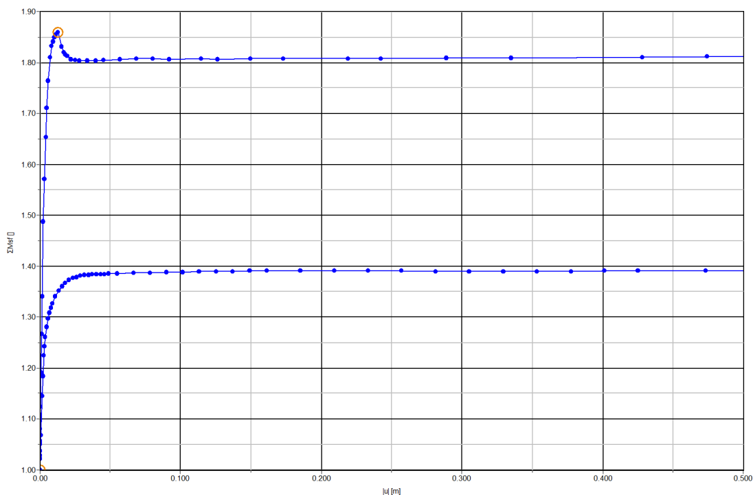
Figure 41: Evaluation of safety factor
