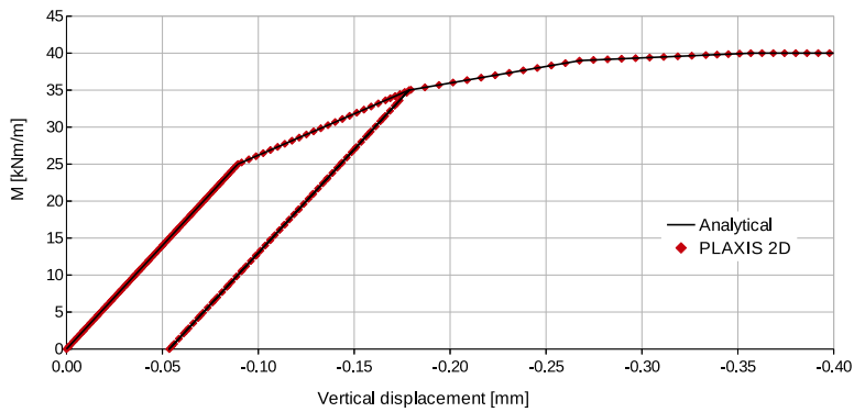
Figure 4 Bending moment versus vertical displacement (load case 3)
