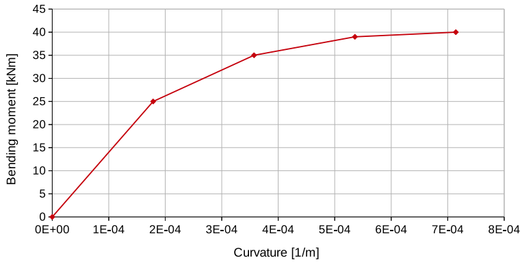
Figure 2 M - \kappa diagram
