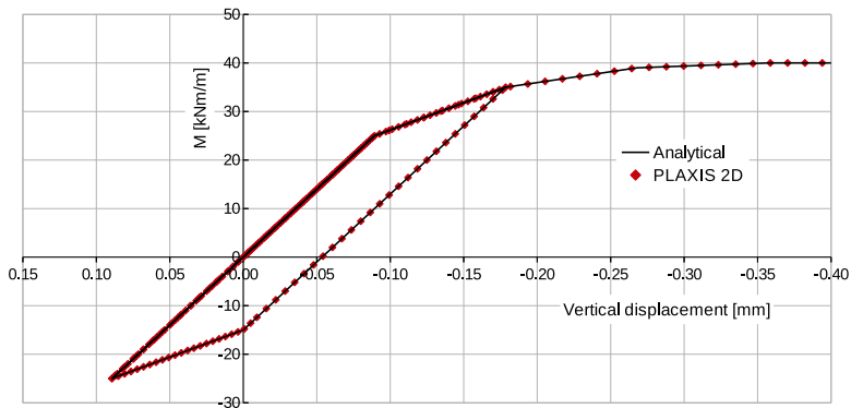
Figure 5 Bending moment versus vertical displacement (load case 4)
