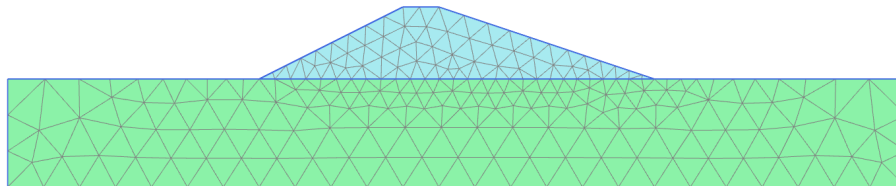
Figure 3: The generated mesh
