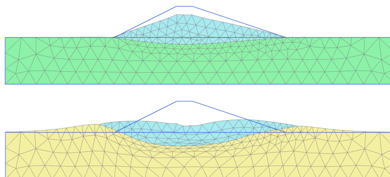
Figure 7: Deformed mesh after phase 1 (top) and phase 2 (bottom)
