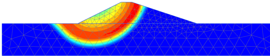
Figure 11: Shadings of the displacement increments indicating the most applicable failure mechanism of the embankment after undrained construction
