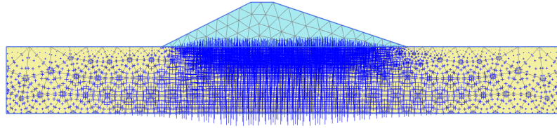
Figure 8: Excess pore pressures after construction on undrained subsoil
