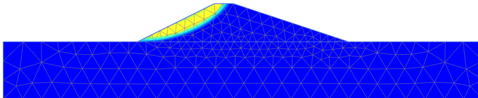
Figure 10: Shadings of the displacement increments indicating the most applicable failure mechanism of the embankment after drained construction
