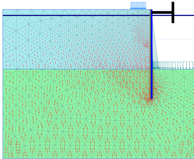
Figure 10: Principal stresses after excavation
