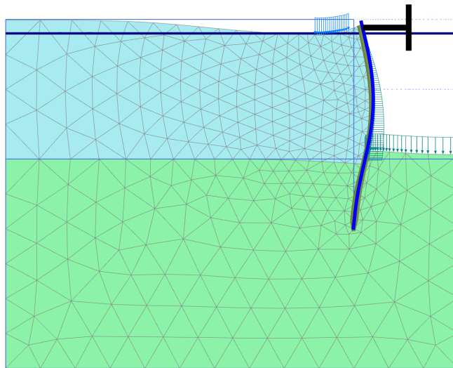
Figure 9: Deformed mesh after the third excavation stage
