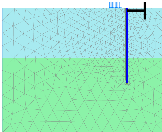
Figure 5: The generated mesh
