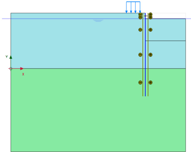
Figure 6: Model view for the first excavation phase
