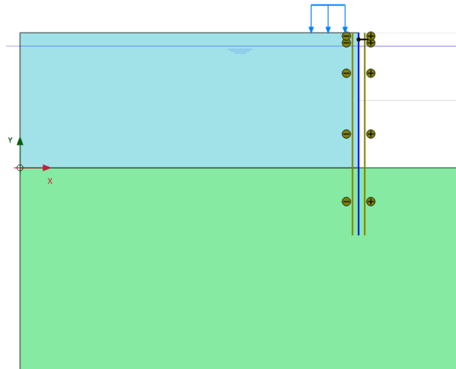
Figure 8: Model view for the third excavation phase
