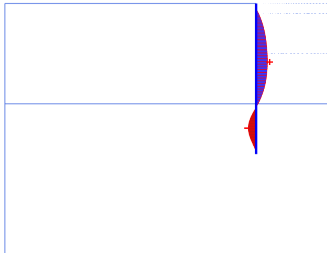
Figure 11: Bending moments in the wall
