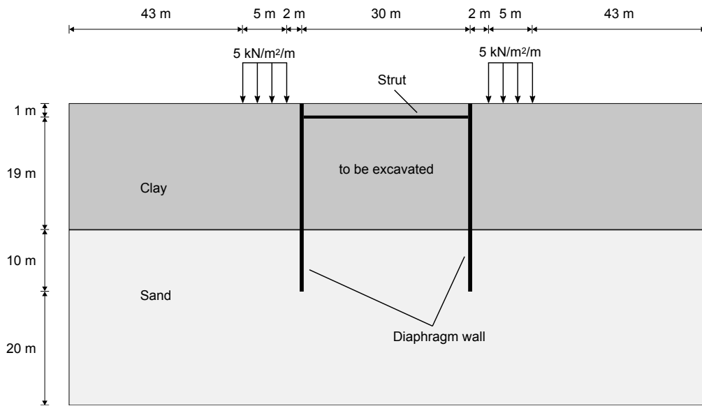
Figure 1: Geometry model of the situation of a submerged excavation
