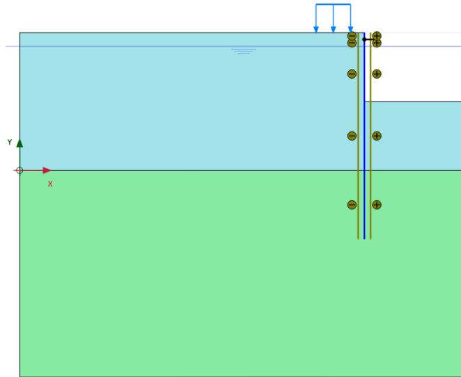
Figure 7: Model view for the second excavation phase
