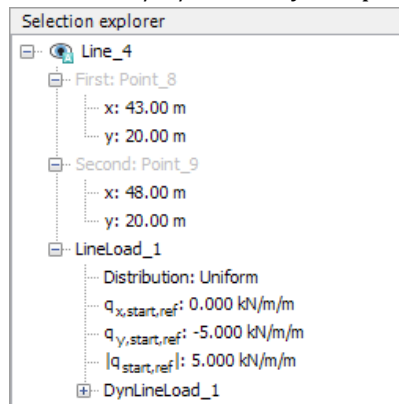
Figure 4: Components of the distributed load in the Selection explorer
