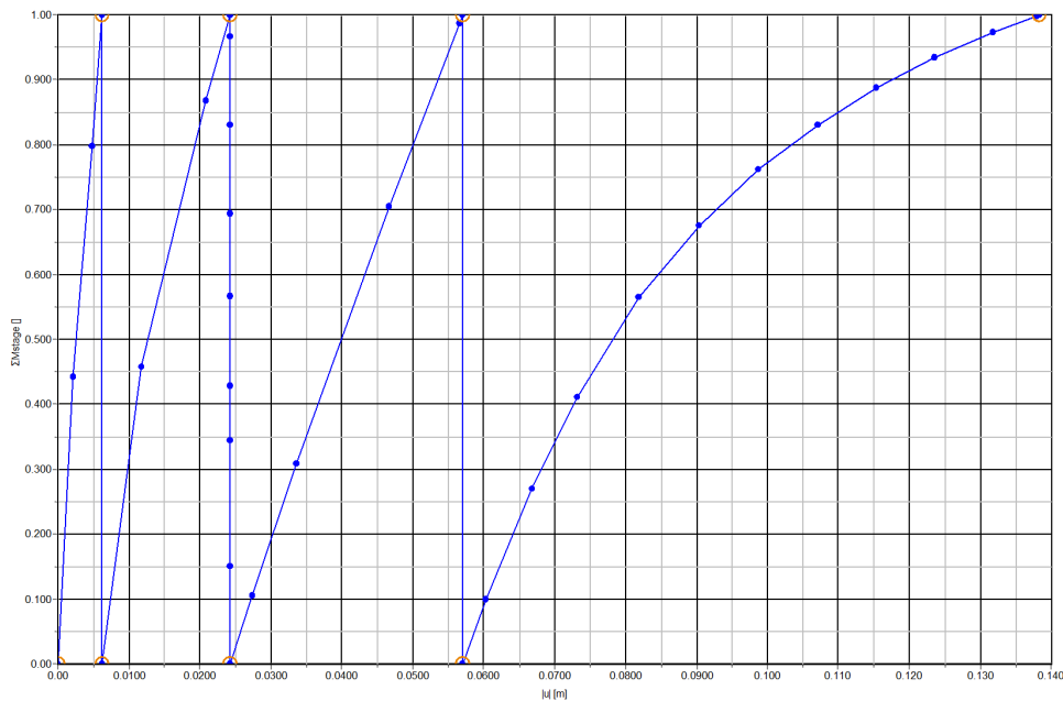
Figure 12: Load-displacement curve of deflection of wall
