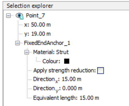
Figure 3: Parameters for fixed-end anchors in the Selection explorer
