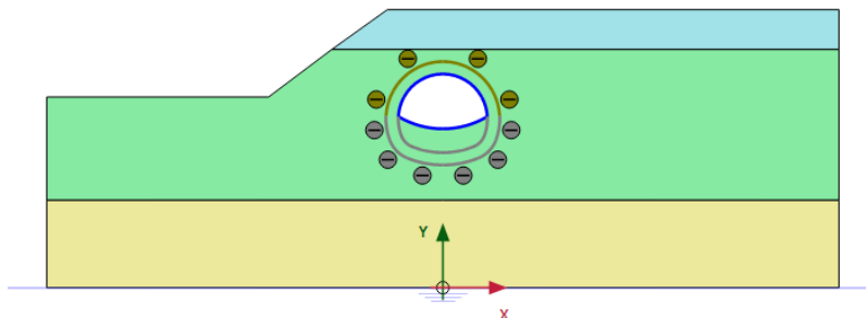
Figure 7: Configuration of Phase 2
