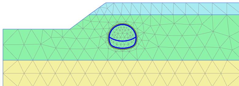
Figure 5: The generated mesh
