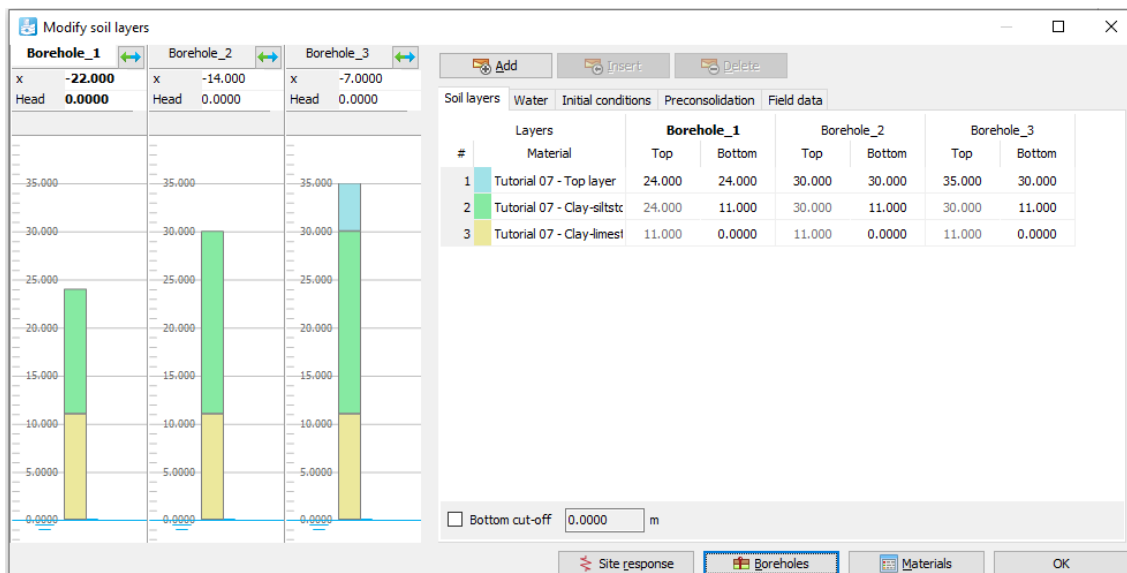
Figure 2: Soil layer distribution
