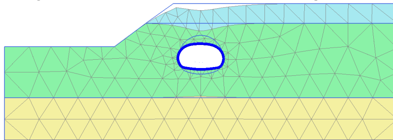
Figure 10: The deformed mesh at the end of the final calculation phase
