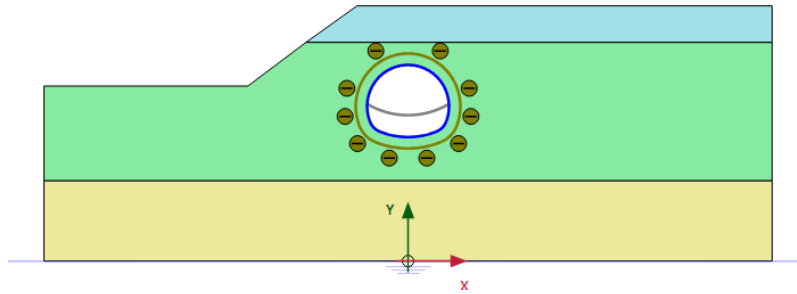
Figure 9: Configuration of Phase 4
