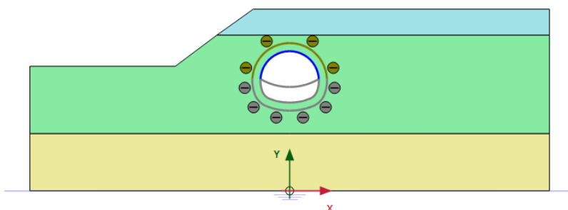
Figure 8: Configuration of Phase 3
