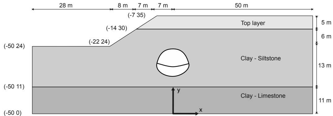
Figure 1: Geometry of the project
