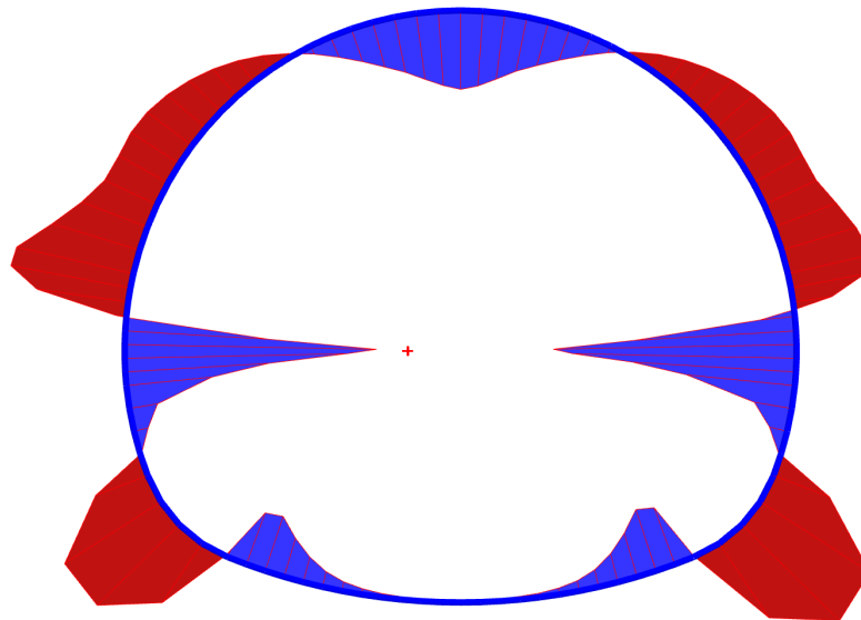
Figure 11: Resulting bending moments in the NATM tunnel
