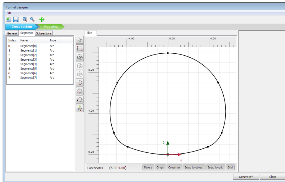
Figure 3: Segments in the tunnel cross section
