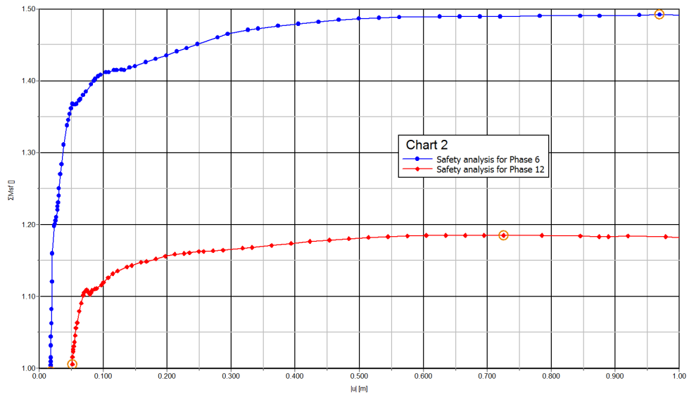
Figure 5: \Sigma M_{sf} - |u| plot for the last calculation phase and the corresponding ULS phase
