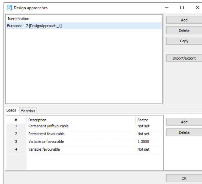
Figure 1: Partial factors for loads
