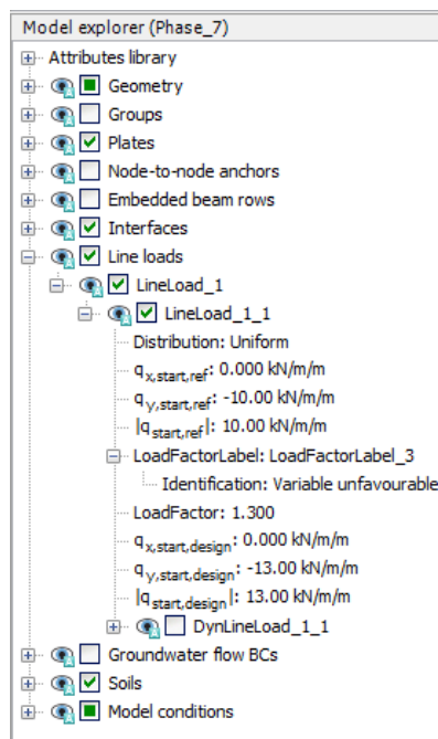
Figure 3: Assignment of factor label to loads in the Selection explorer
