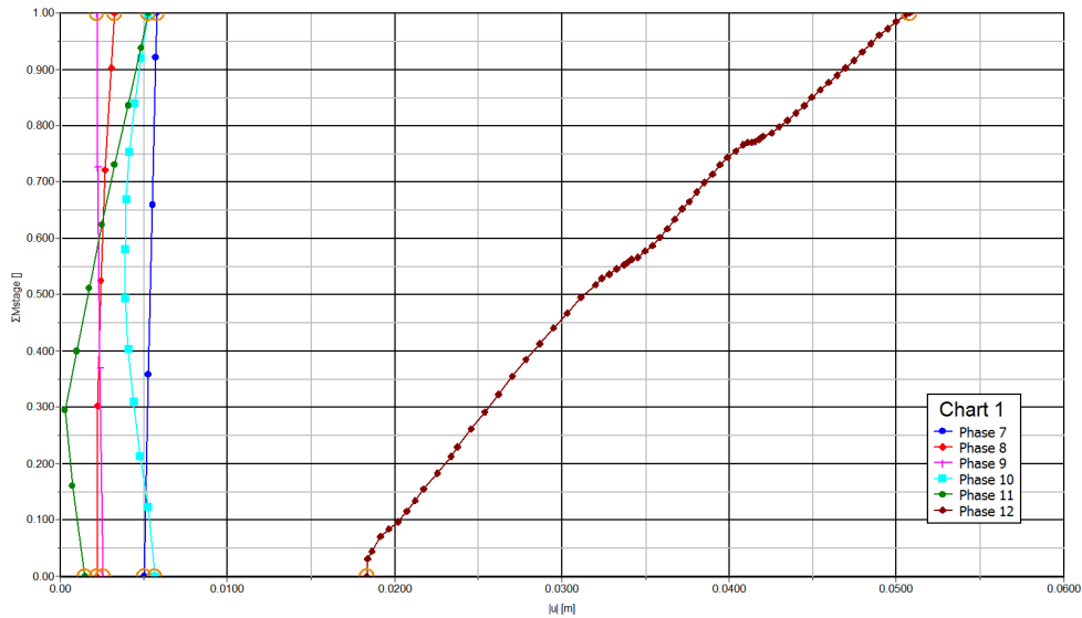
Figure 4: \Sigma M_{stage} - |u| plot for the ULS phases
