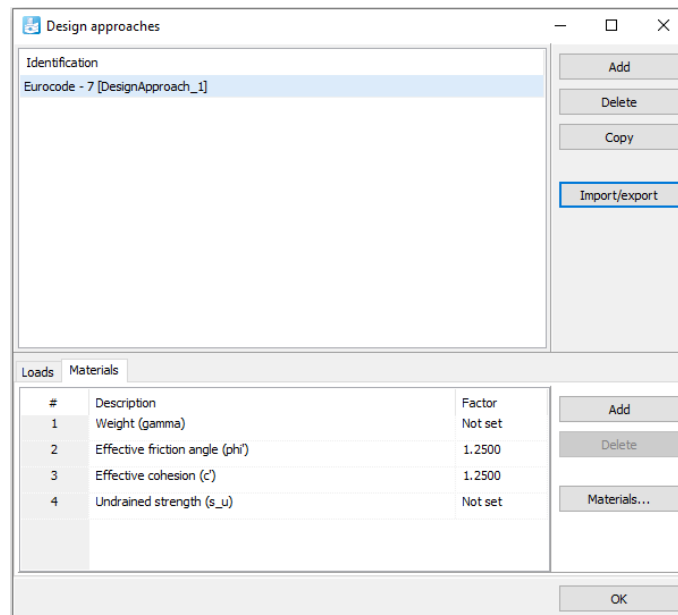
Figure 2: Partial factors for materials
