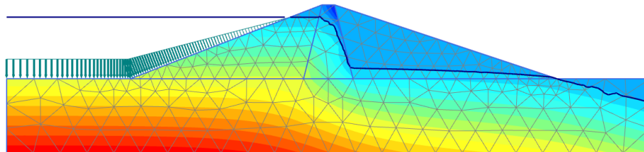
Figure 13: Pore pressure distribution, ( p_{active} ), for high reservoir level
