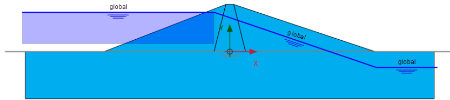
Figure 9: Configuration of the rapid drawdown phase
