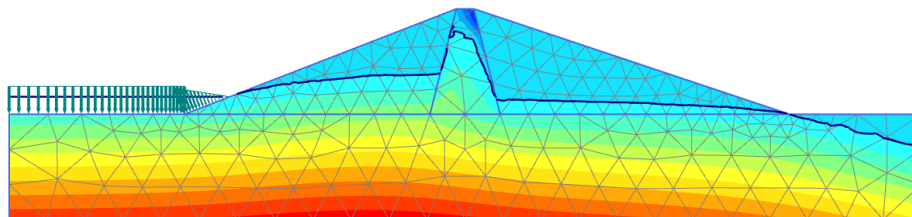
Figure 15: Pore pressure distribution, ( p_{active} ), after slow drawdown
