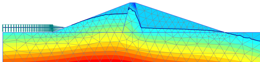
Figure 14: Pore pressure distribution, ( p_{active} ), after rapid drawdown
