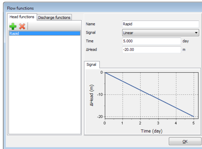
Figure 7: The flow function for the rapid drawdown case
