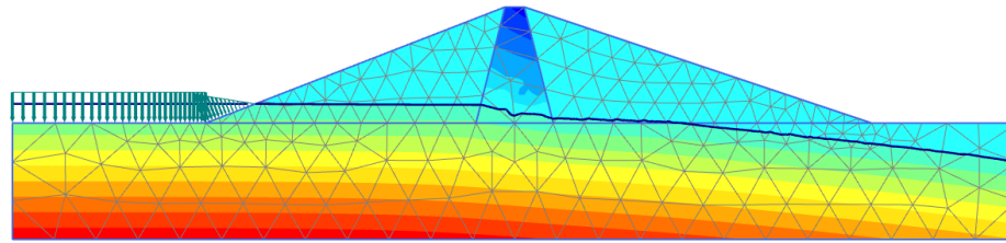
Figure 16: Pore pressure distribution, ( p_{active} ), for low reservoir level
