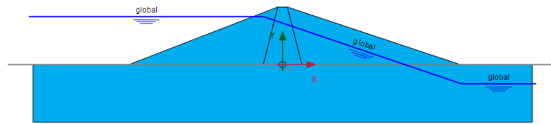
Figure 4: High water level in the reservoir
