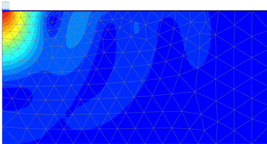
Figure 11: Acceleration ( |a| ) in the soil at the end of phase 2 (with damping)
