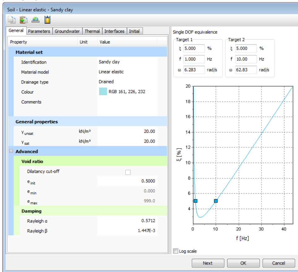
Figure 8: Input of Rayleigh damping
