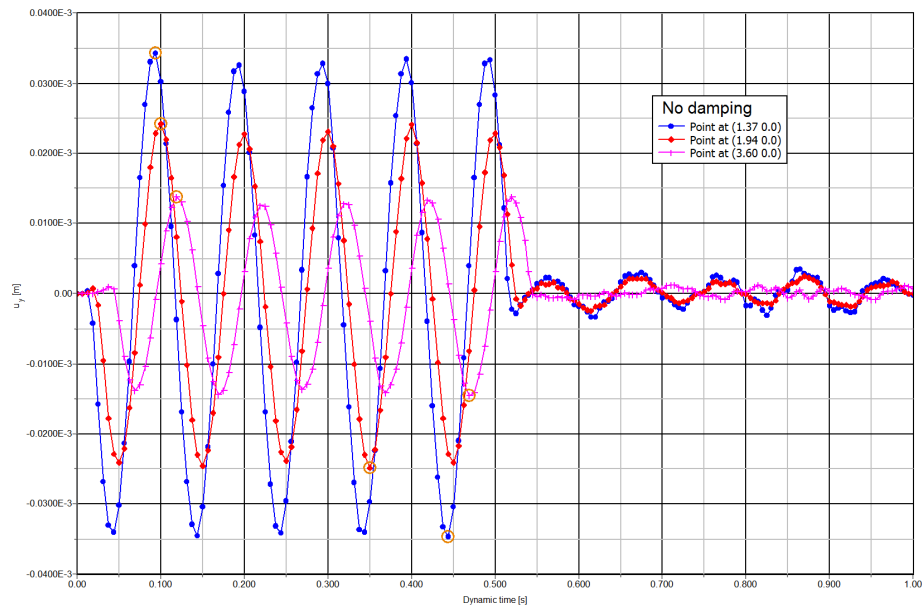
Figure 9: Vertical displ.- time on the surface at different distances to the vibrating source (without damping)
