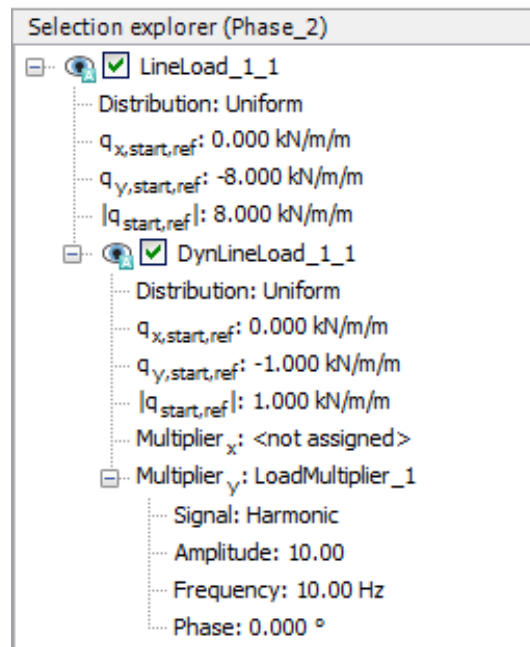
Figure 6: Specification of the dynamic load component in the Selection explorer
