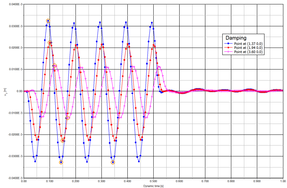
Figure 10: Vertical displ.- time on the surface at different distances to the vibrating source (with damping)
