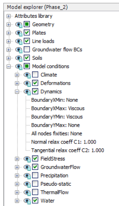
Figure 7: Boundary conditions for dynamics calculations
