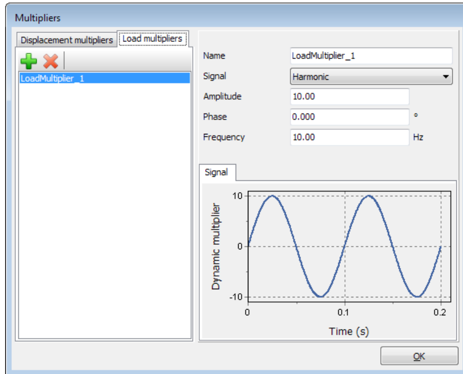
Figure 5: Definition of a Harmonic multiplier
