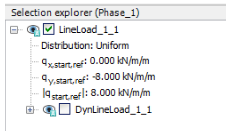
Figure 4: Specification of the static load component in the Selection explorer
