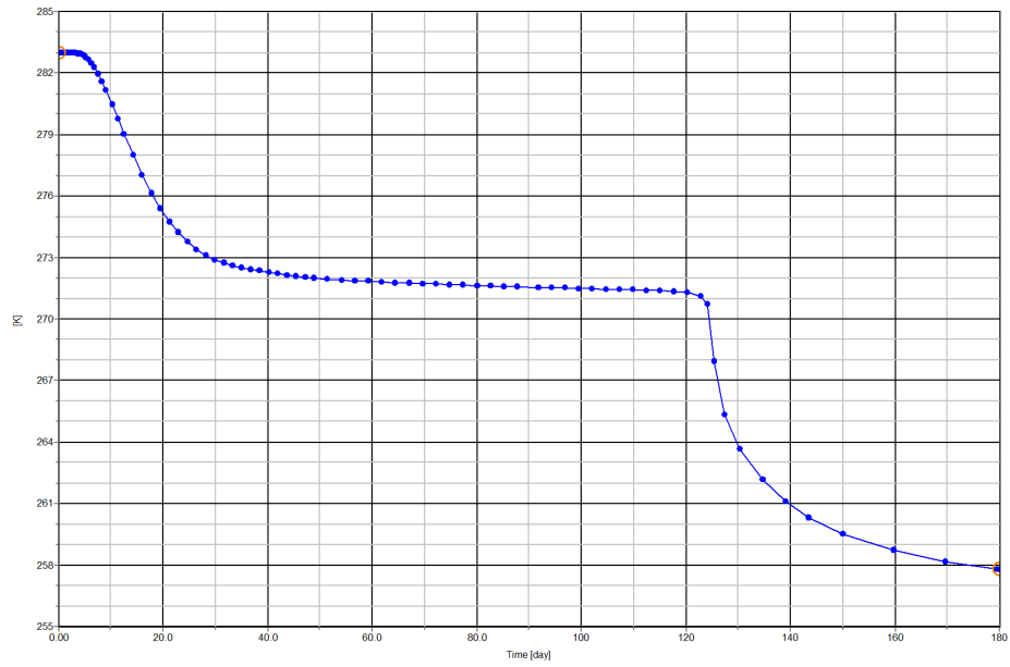
Figure 8: Temperature drop in time at the center of the tunnel
