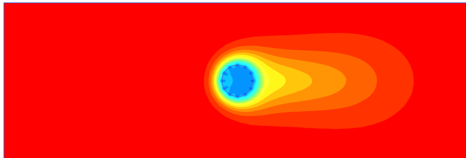
Figure 5: Temperature distribution for transient phase
