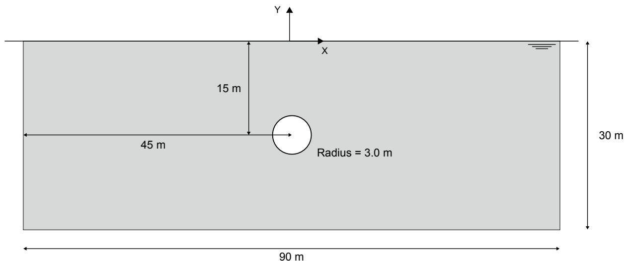
Figure 1: Geometry of the project
