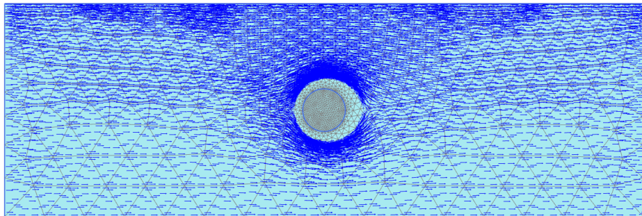
Figure 7: Groundwater flow field after 180 days
