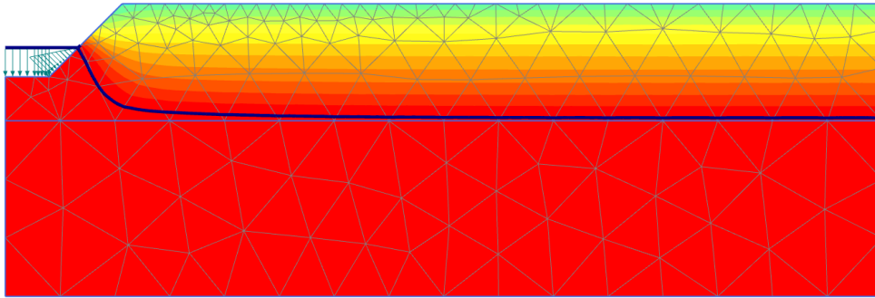
Figure 150: Saturation field at day 15
