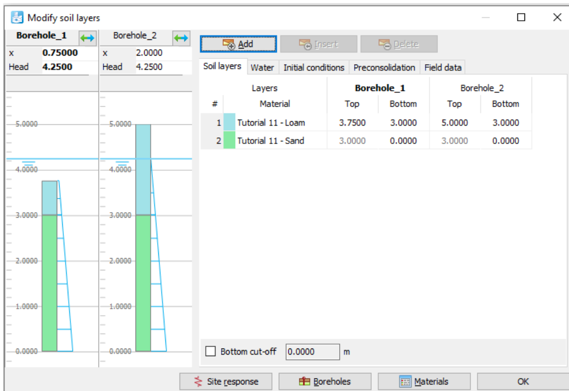
Figure 144: Soil stratigraphy in the Modify soil layers window
