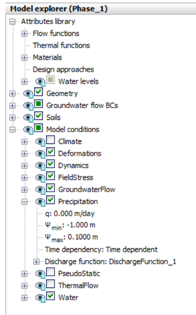
Figure 148: Precipitation in the Model explorer
