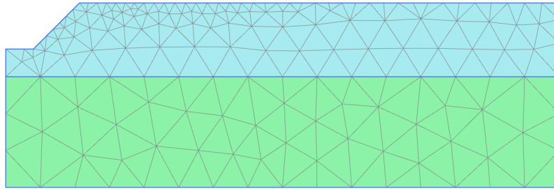
Figure 146: The generated mesh
