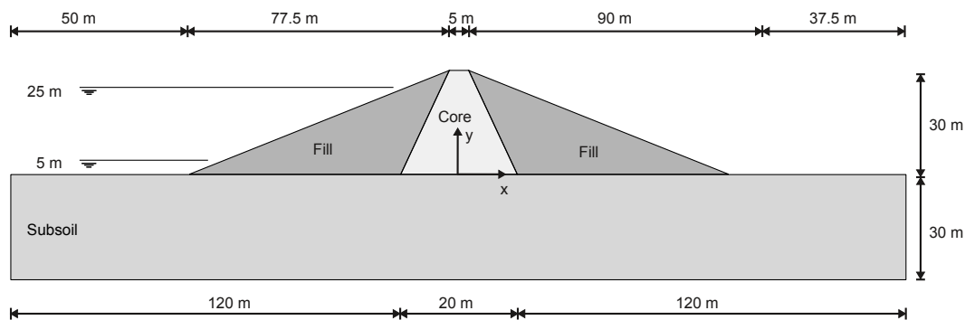
Figure 151: Geometry of the project
