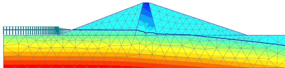
Figure 166: Pore pressure distribution, ( p_{active} ), for low reservoir level
