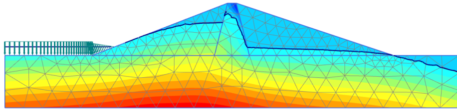
Figure 164: Pore pressure distribution, ( p_{active} ), after rapid drawdown
