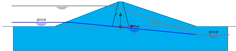
Figure 161: Model for the low level case in the Flow conditions mode
