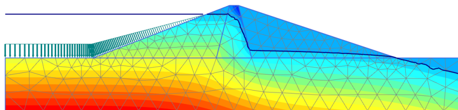
Figure 163: Pore pressure distribution, ( p_{active} ), for high reservoir level
