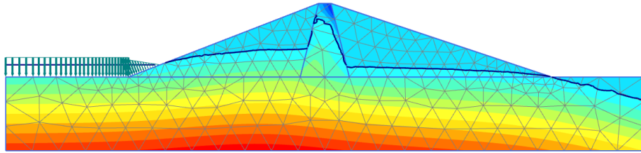
Figure 165: Pore pressure distribution, ( p_{active} ), after slow drawdown
