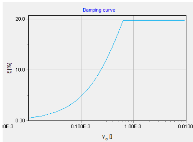
Figure 192: Damping curve for the upper sand layer
