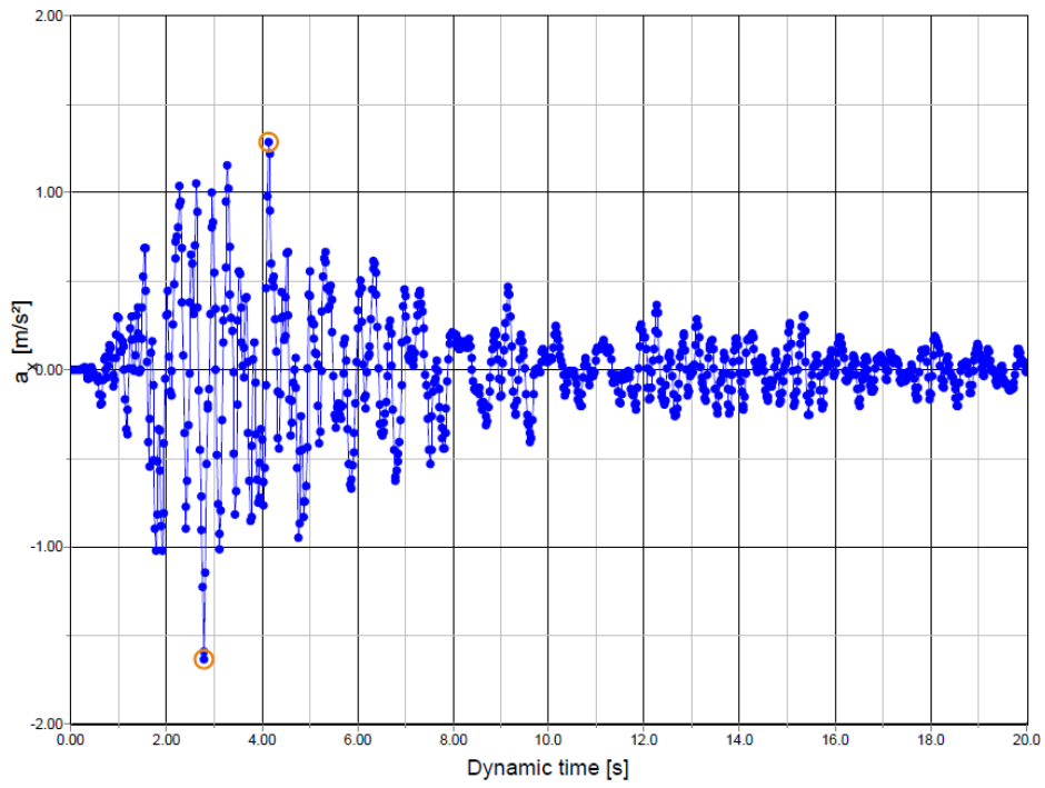
Figure 204: Variation of acceleration in dynamic time
