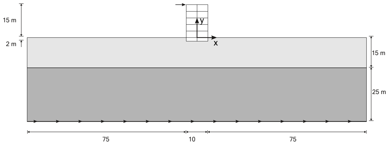
Figure 189: Geometry of the project
