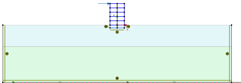
Figure 195: Geometry of the model
