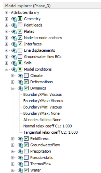
Figure 199: Boundary conditions for dynamics calculations
