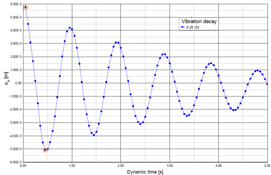
Figure 202: Time history of displacements at selected points
