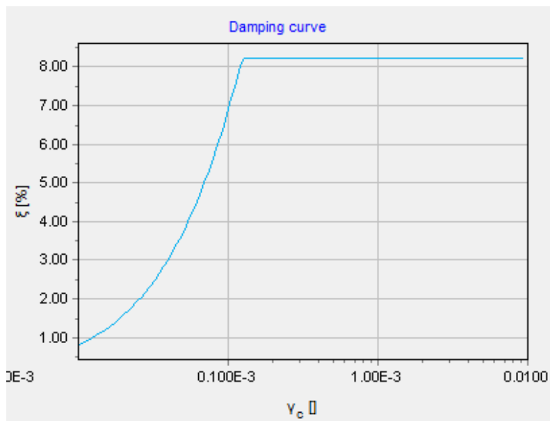
Figure 193: Damping curve for the lower sand layer
