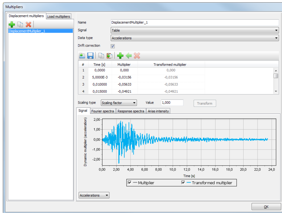
Figure 194: Dynamic multipliers window
