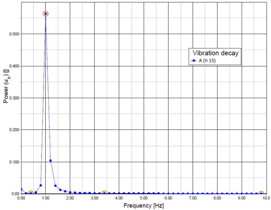
Figure 203: Frequency representation (spectrum)
