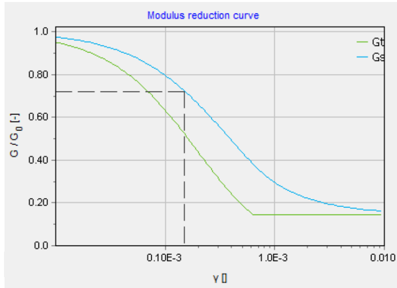
Figure 190: Modulus reduction curves for the upper sand layer
