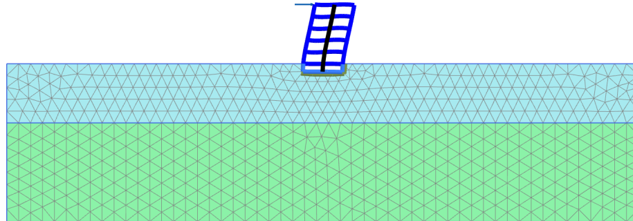
Figure 201: Deformed mesh of the system
