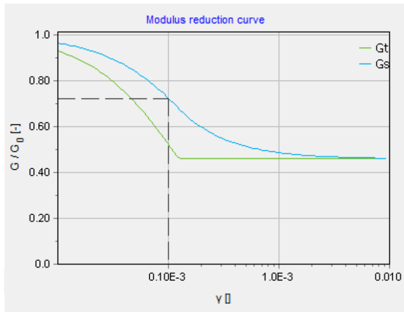
Figure 191: Modulus reduction curve for the lower sand layer
