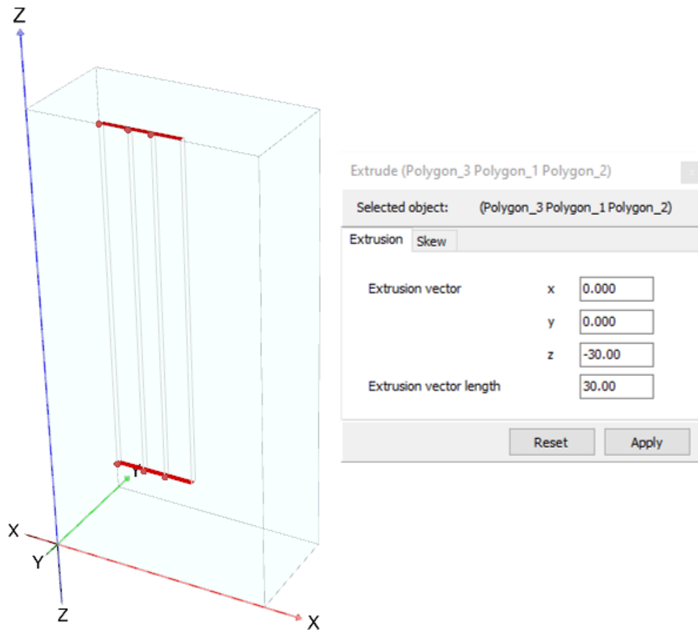
Figure 52: Extruded surfaces
