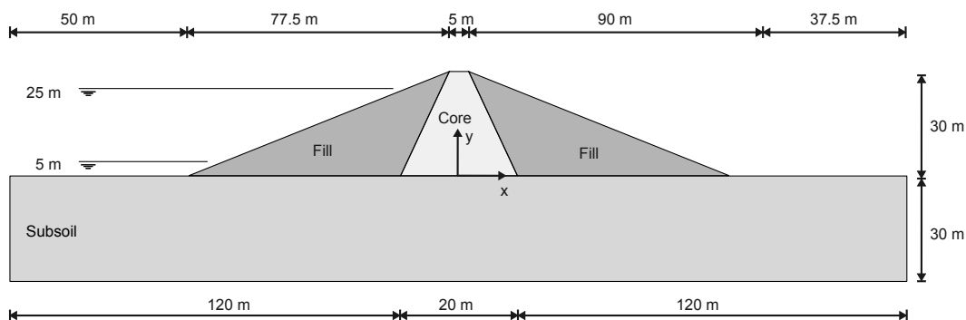
Figure 112: Geometry of the project
