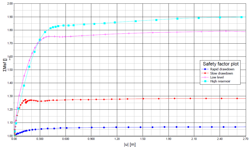
Figure 124: Safety factors for different situations
