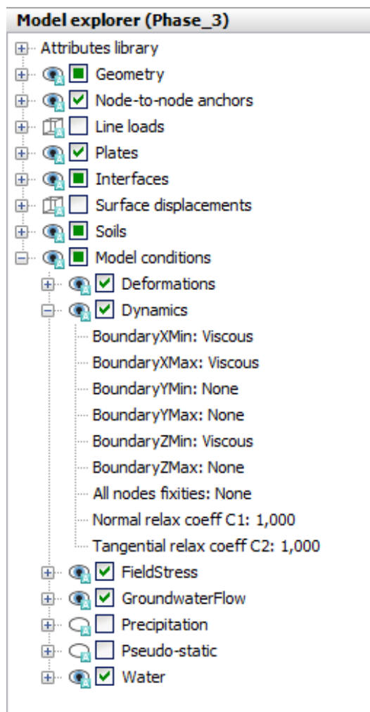
Figure 9: Boundary conditions for dynamics calculations (Phase_3)
