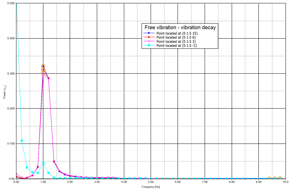
Figure 13: Frequency representation (spectrum - Free vibration)
