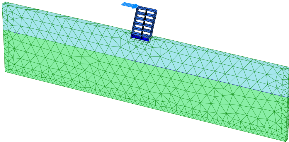
Figure 11: Deformed mesh of the system at the end of Phase_2
