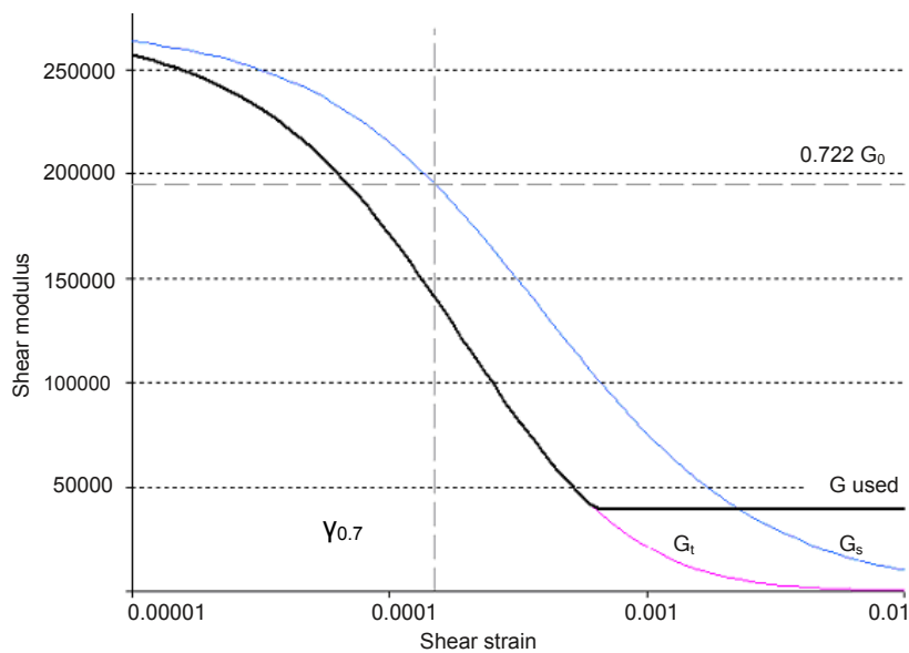
Figure 2: Modulus reduction curves for the upper clayey layer
