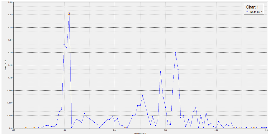
Figure 15: Acceleration power spectra at (0 1.5 15)
