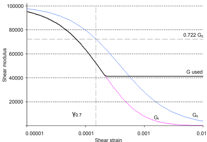
Figure 3: Modulus reduction curve for the lower sandy layer
