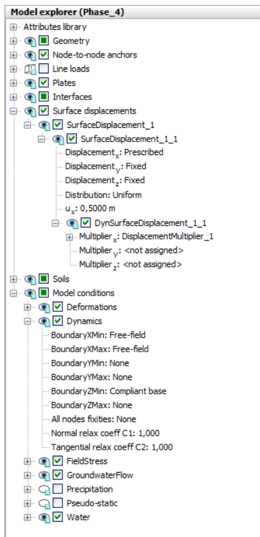
Figure 10: Boundary conditions for dynamics calculations (Phase_4)
