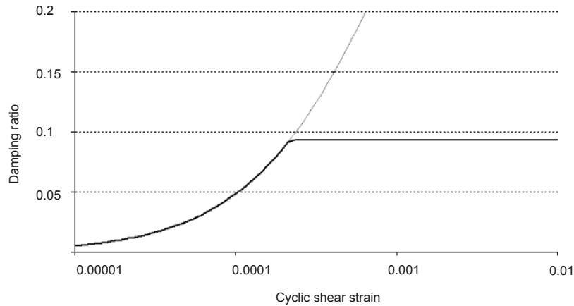
Figure 5: Damping curve for the lower sandy layer
