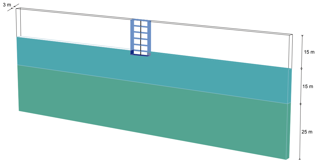
Figure 1: The geometry of the model
