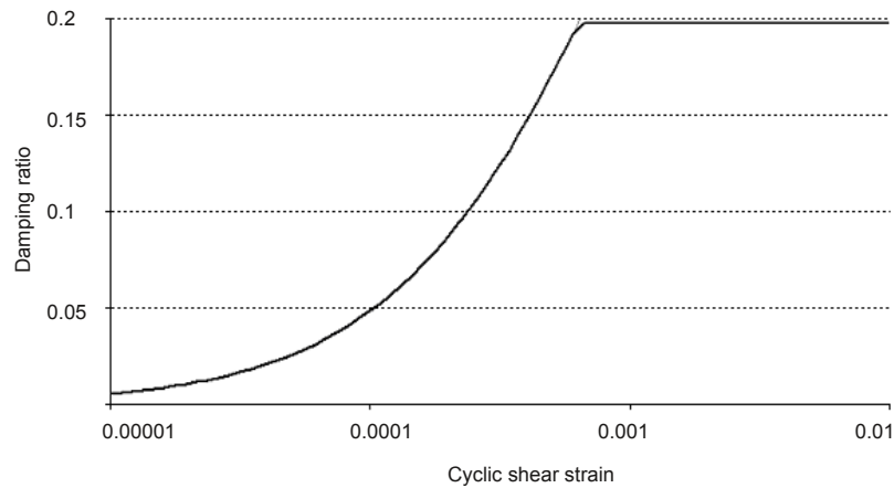
Figure 4: Damping curve for the upper clayey layer
