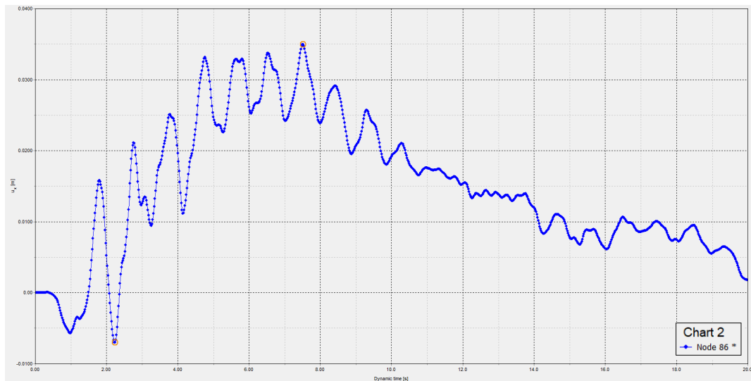
Figure 14: Time history of displacements of the top of the building (Earthquake)
