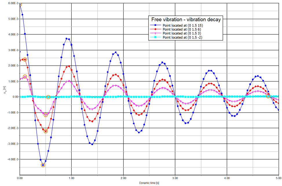
Figure 12: Time history of displacements (Free vibration)
