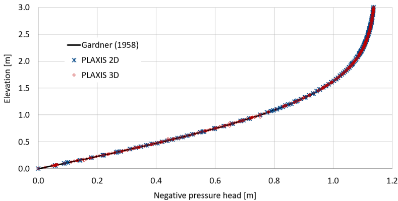
Figure 3 Negative pressure head at steady-state condition
