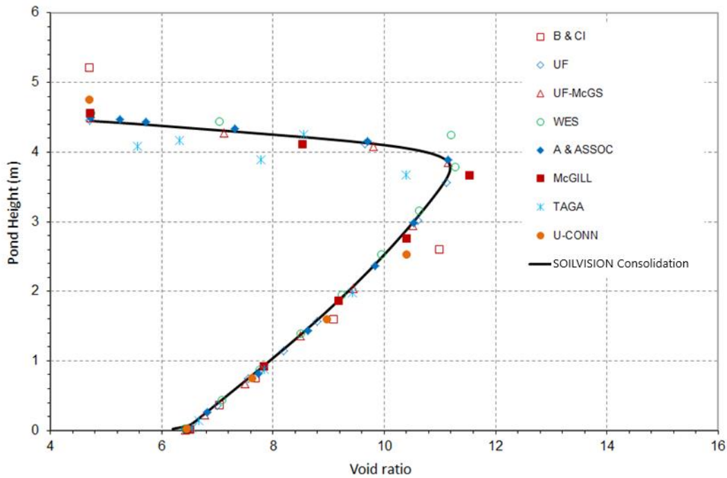
Figure 69: Townsend C 1-year void ratio profile
