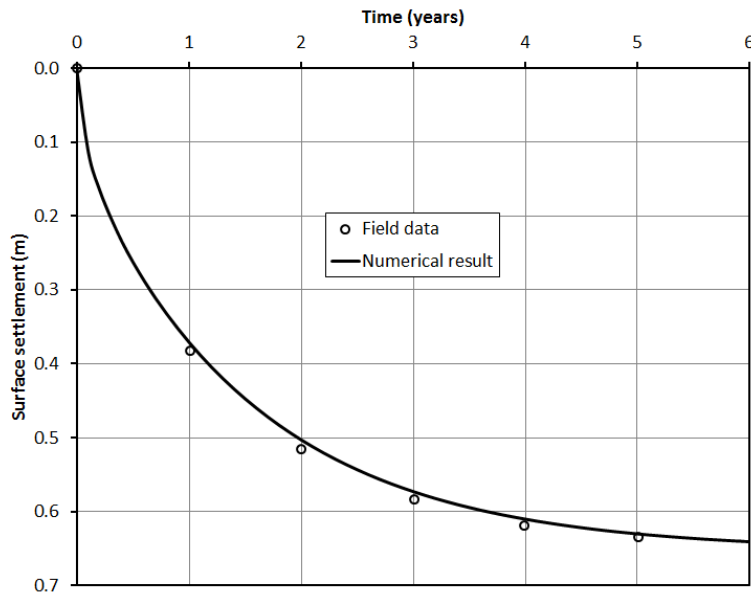
Figure 11. Settlement with time: PLAXIS LE Consolidation numerical result and data reported by Lambe and Whitman (1969).
