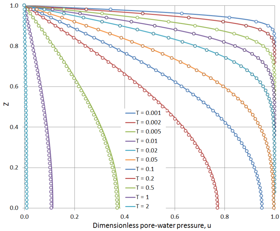
Figure 2. Dimensionless pore-water pressure profile at various dimensionless time factors, T . The marker points are the closed-form solution and solid lines are the PLAXIS LE Consolidation solution.
