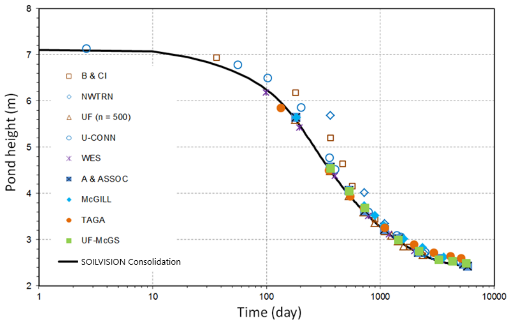
Figure 67: Townsend C settlement of tailings over time
