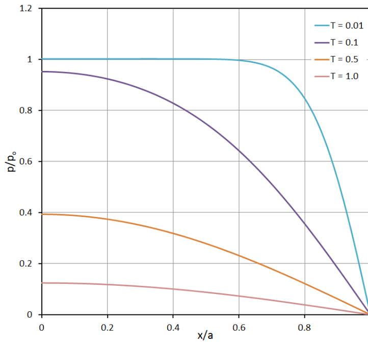
Figure 28. Normalized excess pore-water pressure along the base with Poisson ratio = 0.49 (Problem 1).
