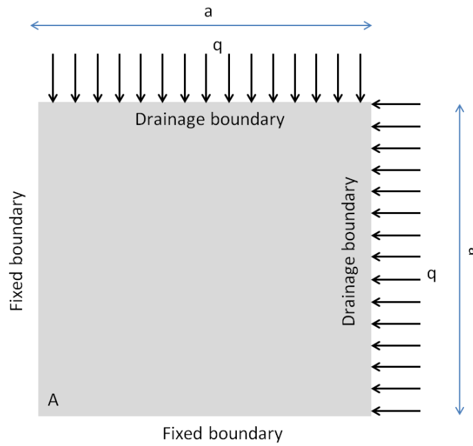
Figure 24. Geometry and boundary conditions (Problem 2)
