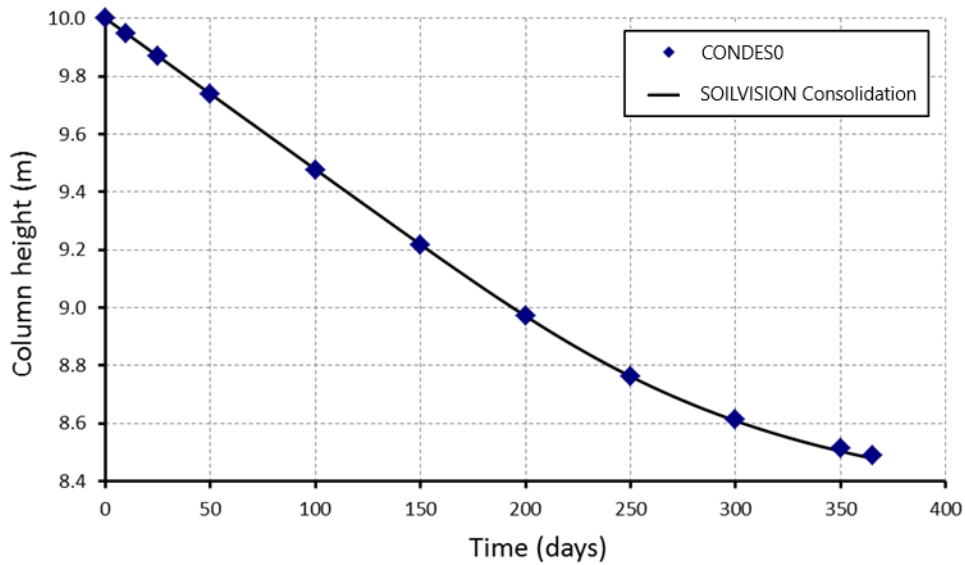
Figure 42: Column height comparison between PLAXIS LE Consolidation and CONDES0
