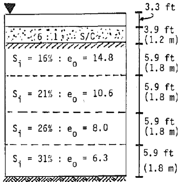
Figure 70: Townsend's Scenario D (from Townsend & McVay, 1990).
