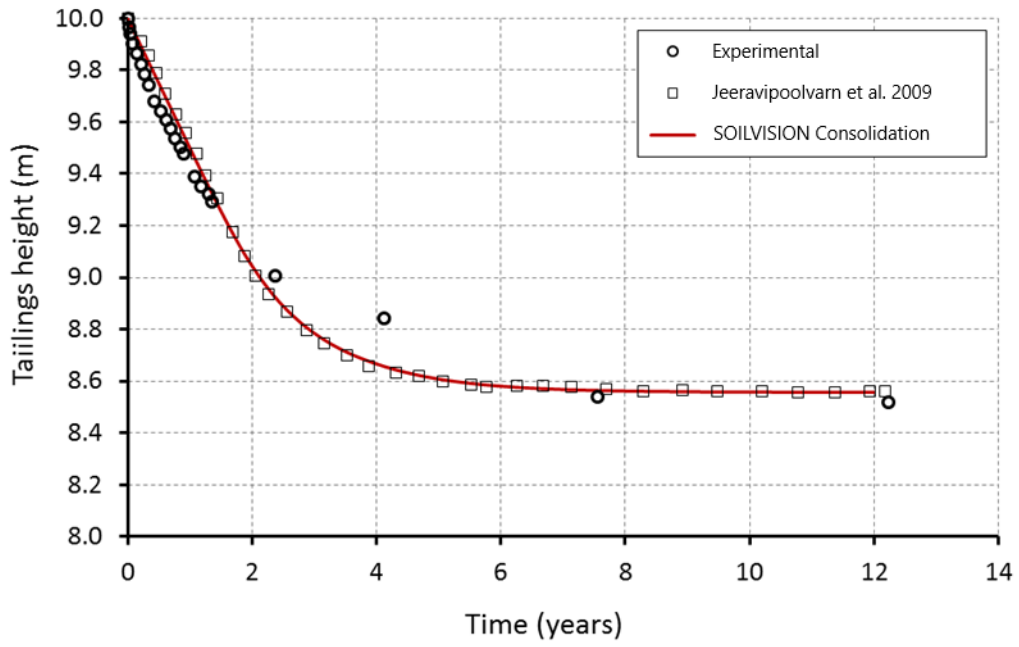
Figure 52 Column 3 settlement results
