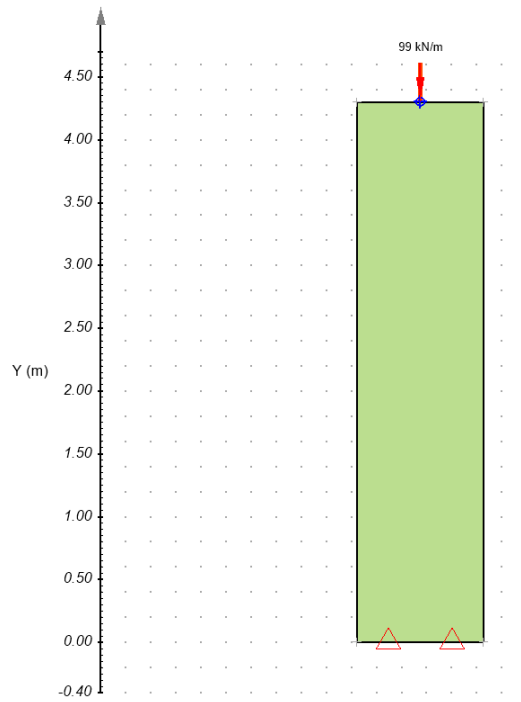
Figure 10. Geometry of model in PLAXIS LE Consolidation
