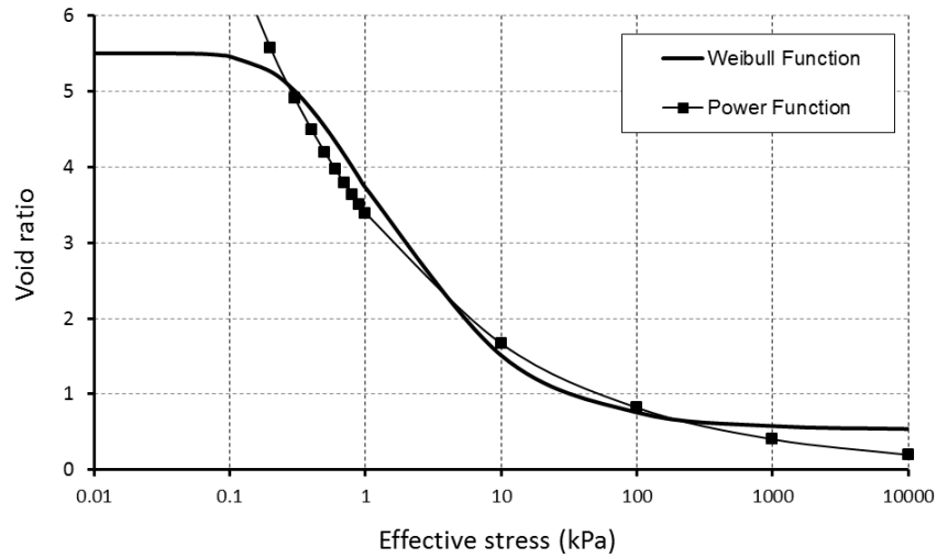
Figure 44. Weibull and Power functions utilized in the PLAXIS LE Consolidation Standpipe 1 numerical model for compressibility relationship
