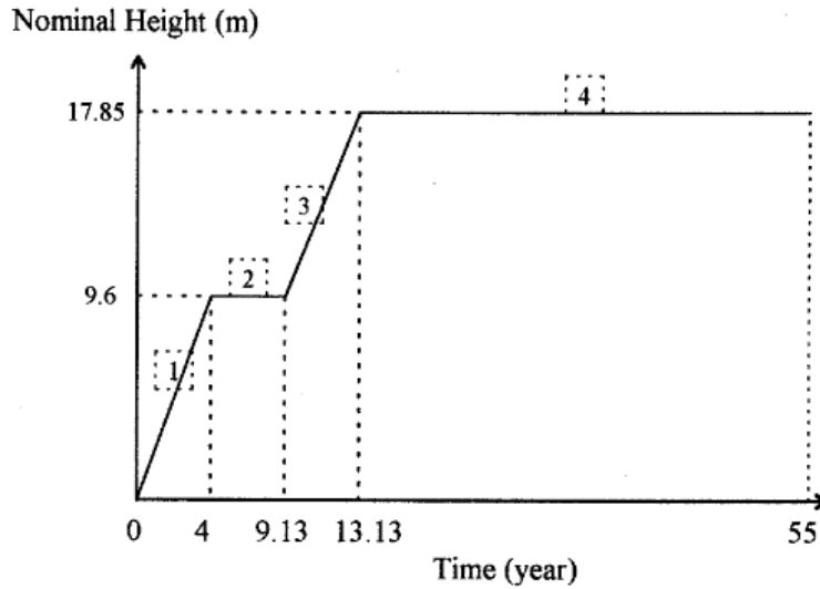
Figure 80: CONDES0 - Example 3 nominal height vs time plot (from Yao & Znidarčić, 1997)
