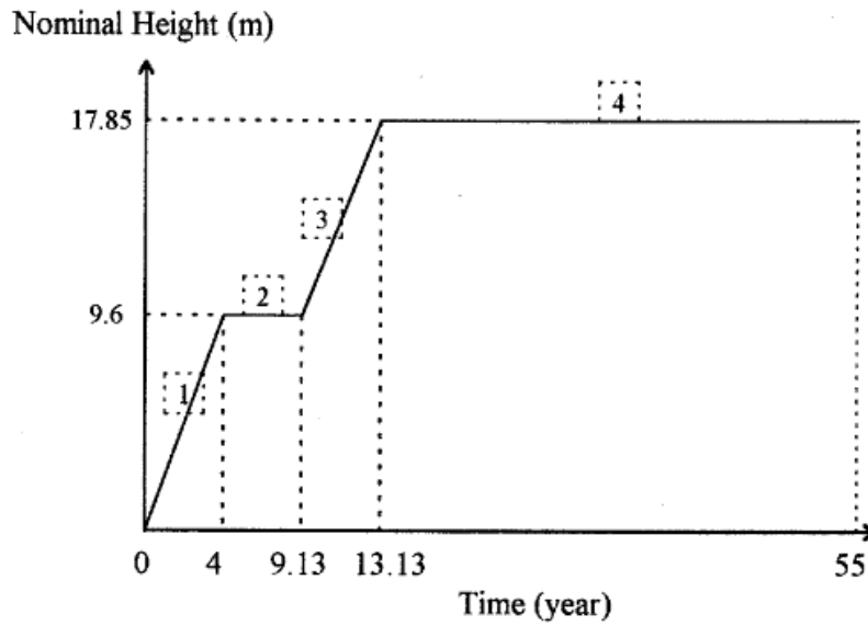
Figure 77: CONDES0 - Example 2 nominal height vs time plot (from Yao & Znidarčić, 1997)
