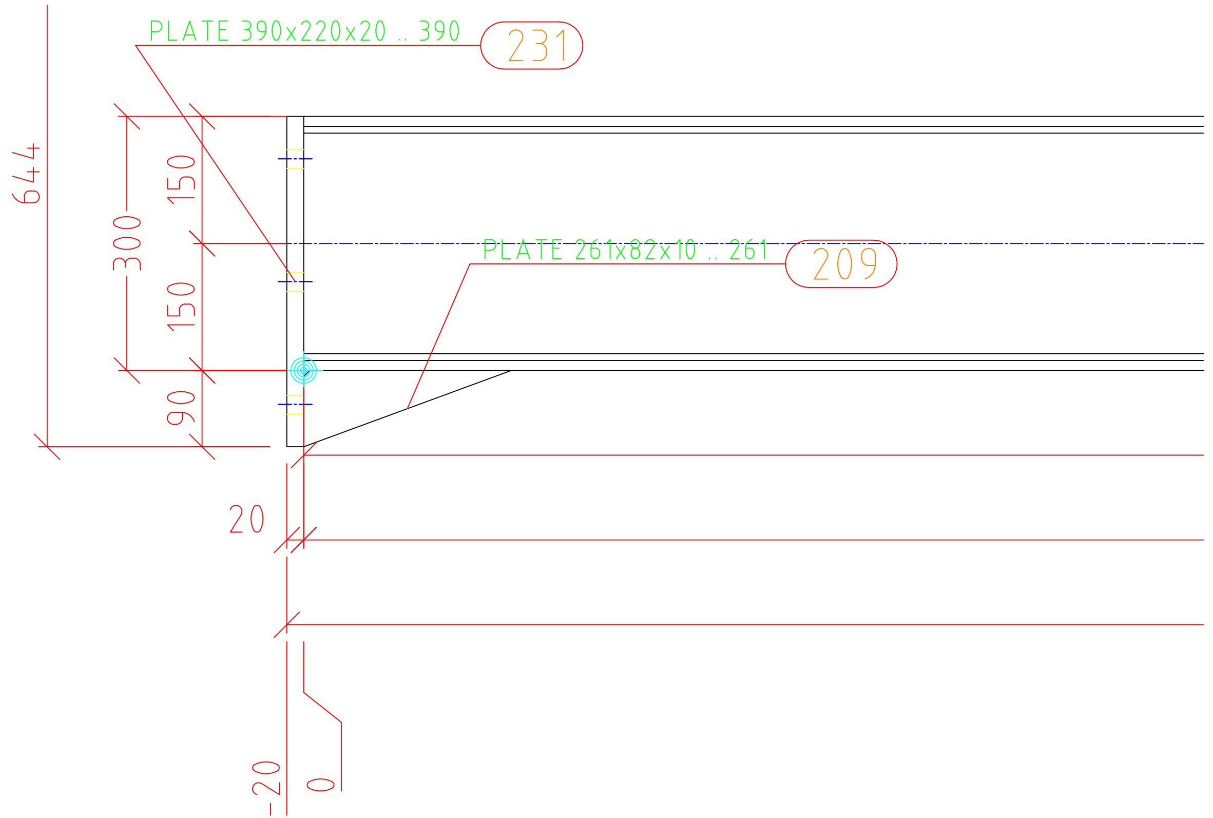
Pos. GR. 10 Front View (Sc1:10) IPN 300 (1 x) Length:4628
